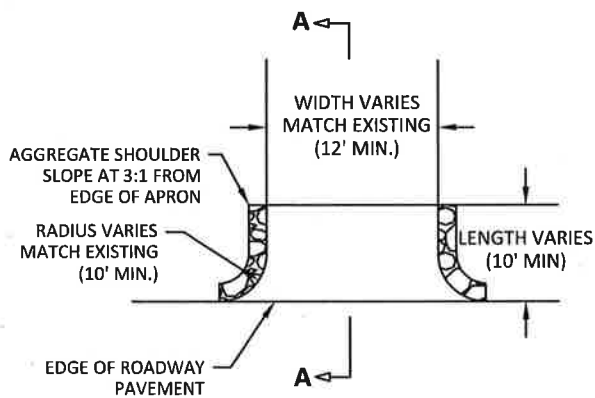
DRIVEWAY APRON DETAIL
