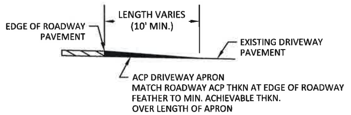
SECTION A-A (EXISTING PAVED APPROACH)
