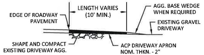
SECTION A-A (EXISTING GRAVEL APPROACH)
