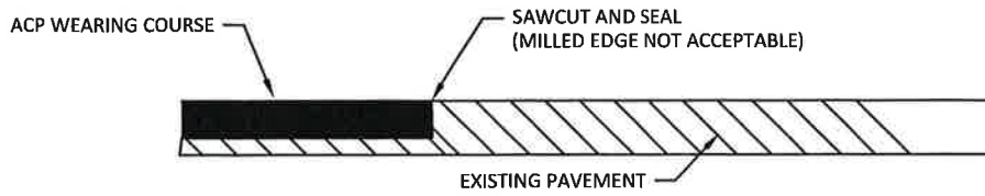
COLD PLANE REMOVAL EDGE DETAIL
