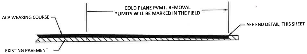
0"-2" COLD PLANE REMOVAL DETAIL PROFILE VIEW
