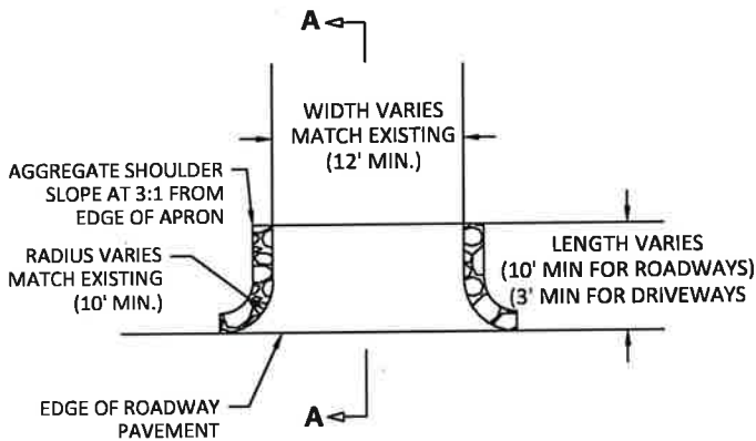
INTERSECTION APPROACH AND DRIVEWAY APRON DETAIL
