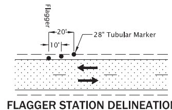
FLAGGER STATION DELINEATION
