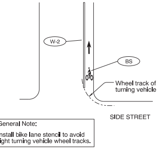
INSTALLATION OF BIKE LANE STENCILS FOLLOWING INTERSECTIONS
